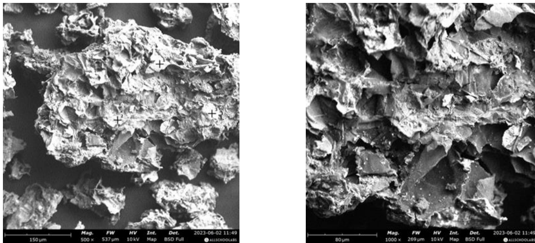
Fig. 5. (A-B). SEM Spectrum of 500 and 1000 Mag for Silver Oxide nano-particle-Avocado Pear Seed (AgAPS)
