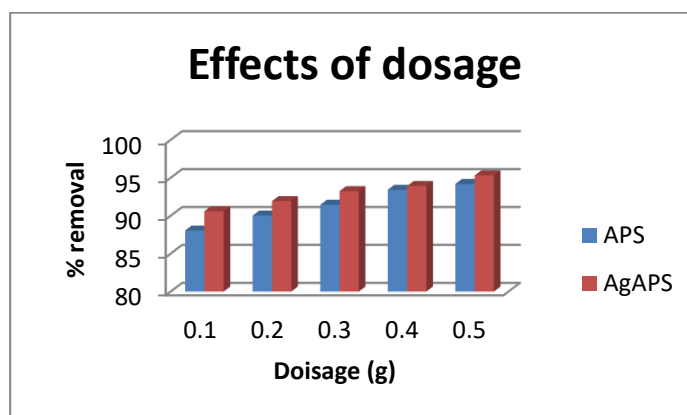
Fig. 8. Effects of dosage on the percentage removal of copper onto avocado pear seed
