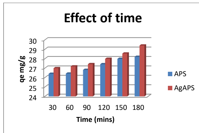
Fig. 6. Effect of time on the adsorption of copper onto avocado pear seed
