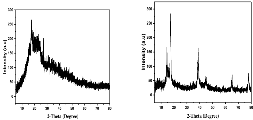
Fig. 3. XRD Spectroscopic Spectrum for avocado pear seed (APS) Fig 4. XRD Spectroscopic Spectrum for Silver Oxide nano-particle-Avocado Pear Seed (AgAPS)
