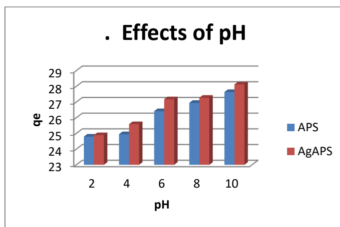
Fig. 7. Effects of pH on the adsorption of copper onto avocado pear seed
