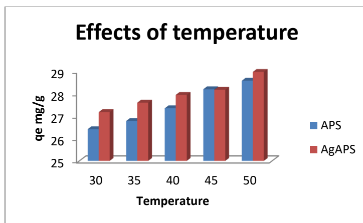
Fig. 9. Effects of temperature on the adsorption of copper onto avocado pear seed
