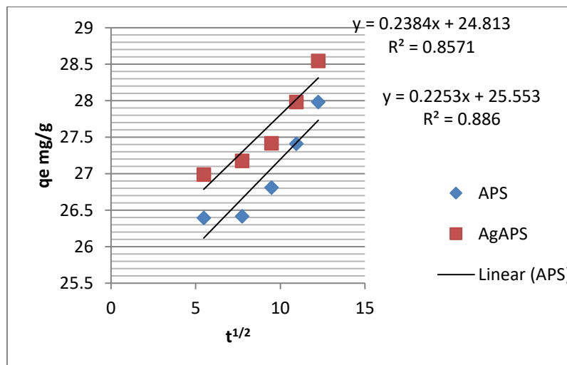
Fig. 12. Intra-particle diffusion plot for the adsorption of copper onto avocado pear seed
